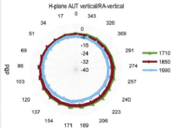
estimated gain (dBd) 1800/1900 MHz band
