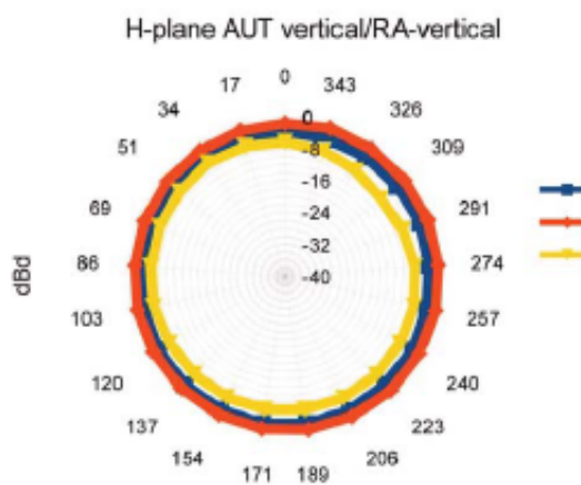
estimated gain (dBd) 850/900 MHz band
